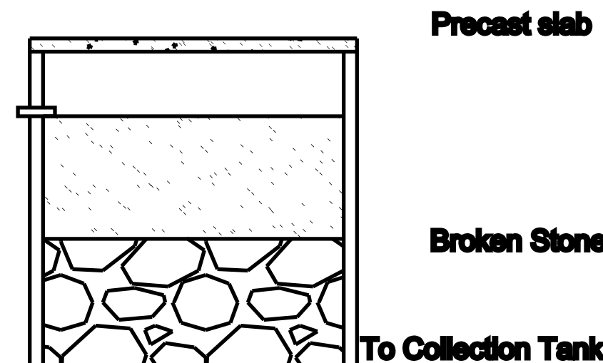
Section of Filter Unit
