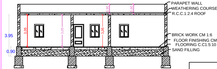
SECTION ON SV
