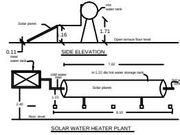
SOLAR WATER HEATER PLANT
