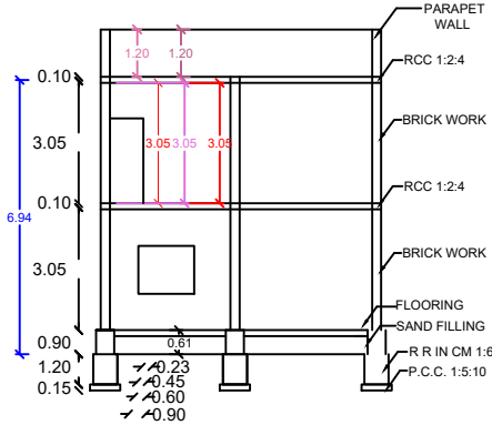
SECTION AB
