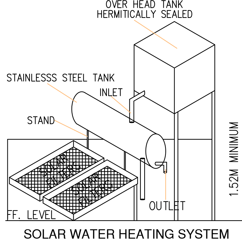
SOLAR WATER HEATING SYSTEM
