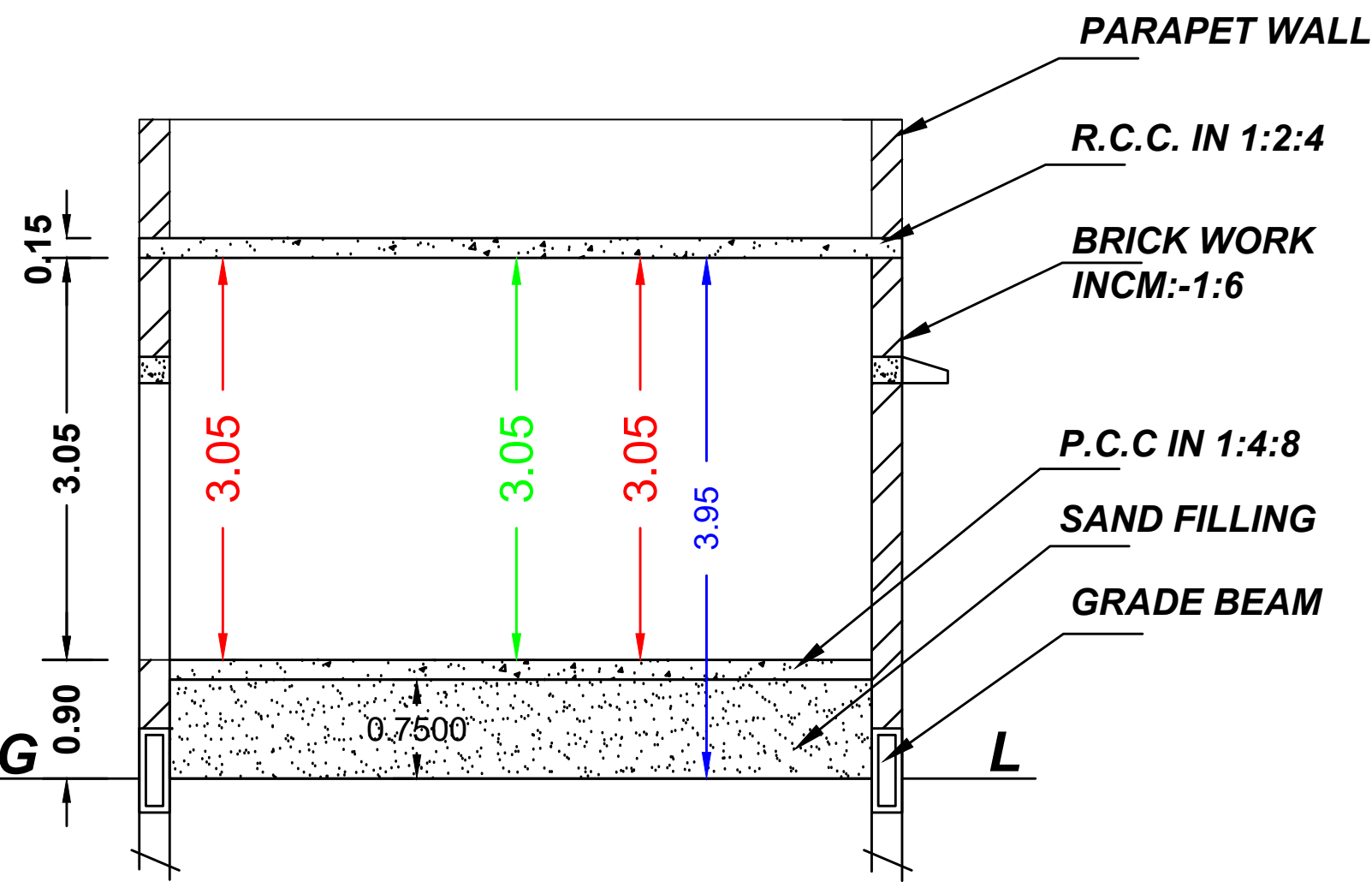
SECTION "AB"
