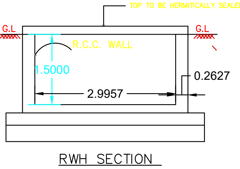
RWH SECTION
