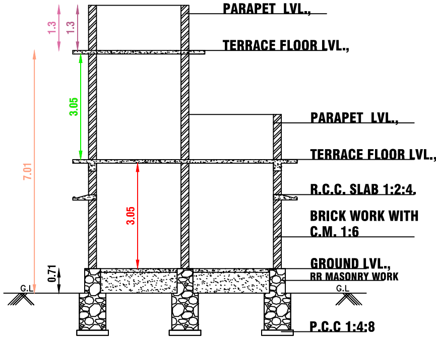
SECTION ON A-A & A'-A'
