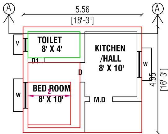
EX. GROUND FLOOR PLAN
