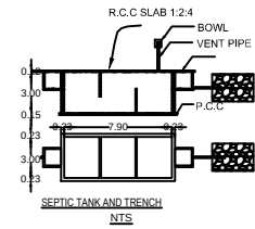
SEPTIC TANK AND TRENCH NTS
