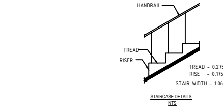
STAIRCASE DETAILS NTS
