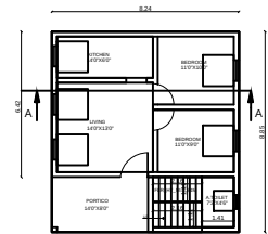
GF PLAN
