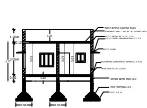
SECTIONON-AA
