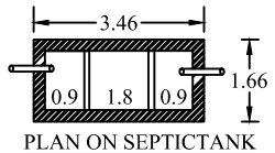
PLAN ON SEPTICTANK
