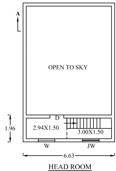
HEAD ROOM
