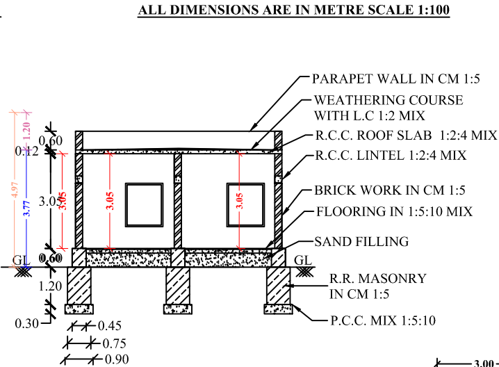
SECTION OF "AB"
