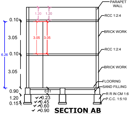
SECTION AB
