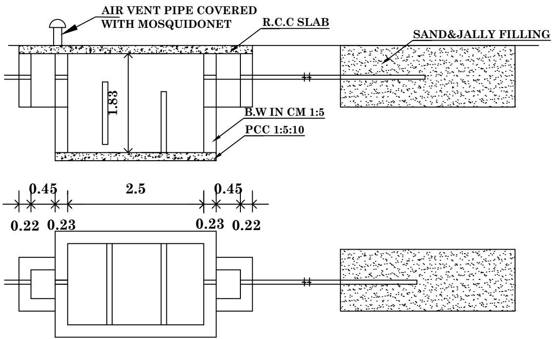
PLAN&SECTION OF SEPTIC TANK TRENCH
