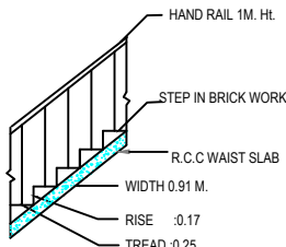
STAIR DETAIL
