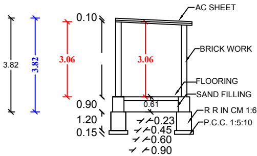
SECTION AB
