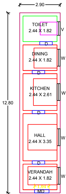
PLAN
