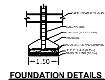
FOUNDATION DETAILS
