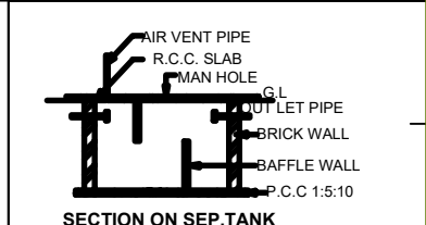
SECTION ON SEPT.TANK
