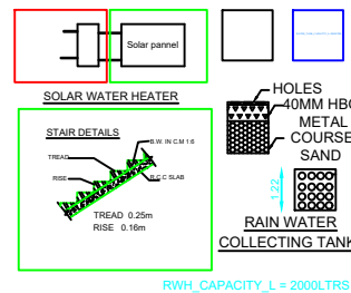
RWH_CAPACITY_L = 2000LTRS
