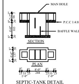
SEPTIC-TANK DETAIL
