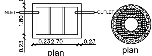
LEACH WELL DETAIL
