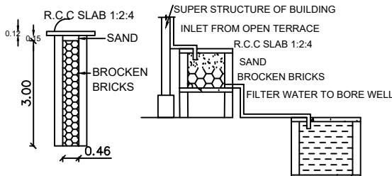
DETAILS OF FILTER BED & WELL
