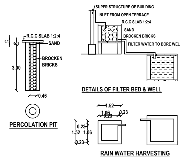
RAIN WATER HARVESTING
