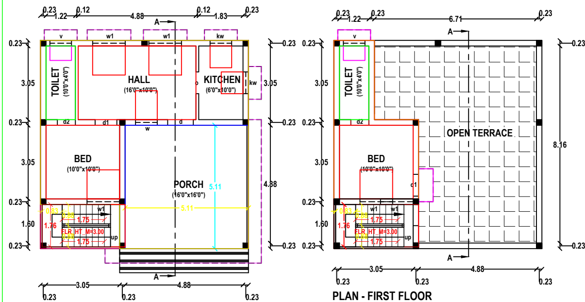
PLAN - GROUND FLOOR RESIDENCE
