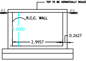
RWH SECTION
