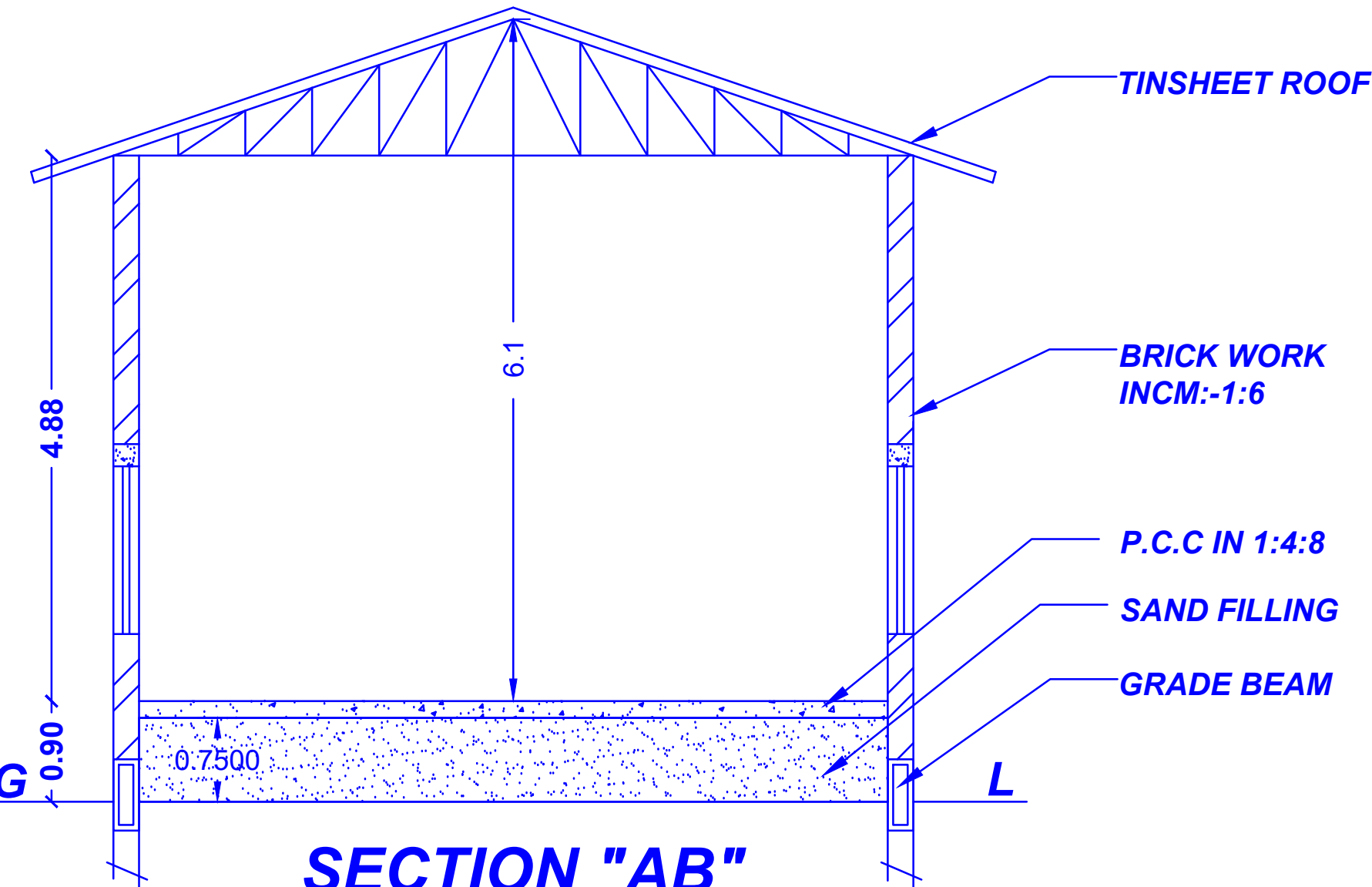
SECTION "AB"
