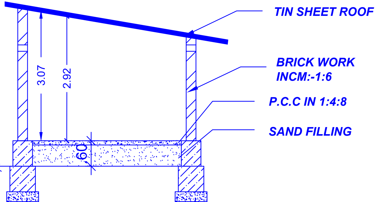
SECTION "AB"
