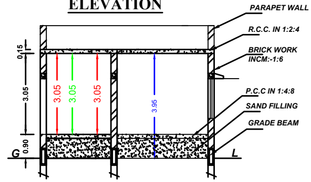
SECTION "AB"
