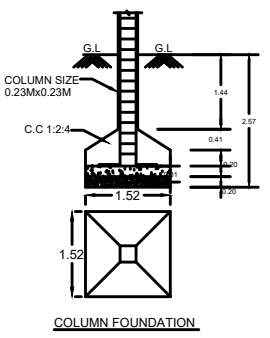
COLUMN FOUNDATION
