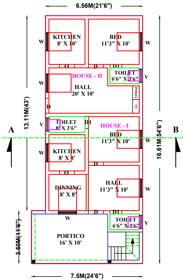
PLAN
