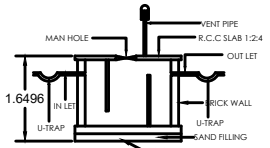
SECTION E.F SEPTIC TANK DETAIL
