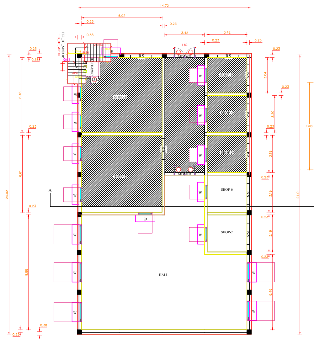
GF PLAN
