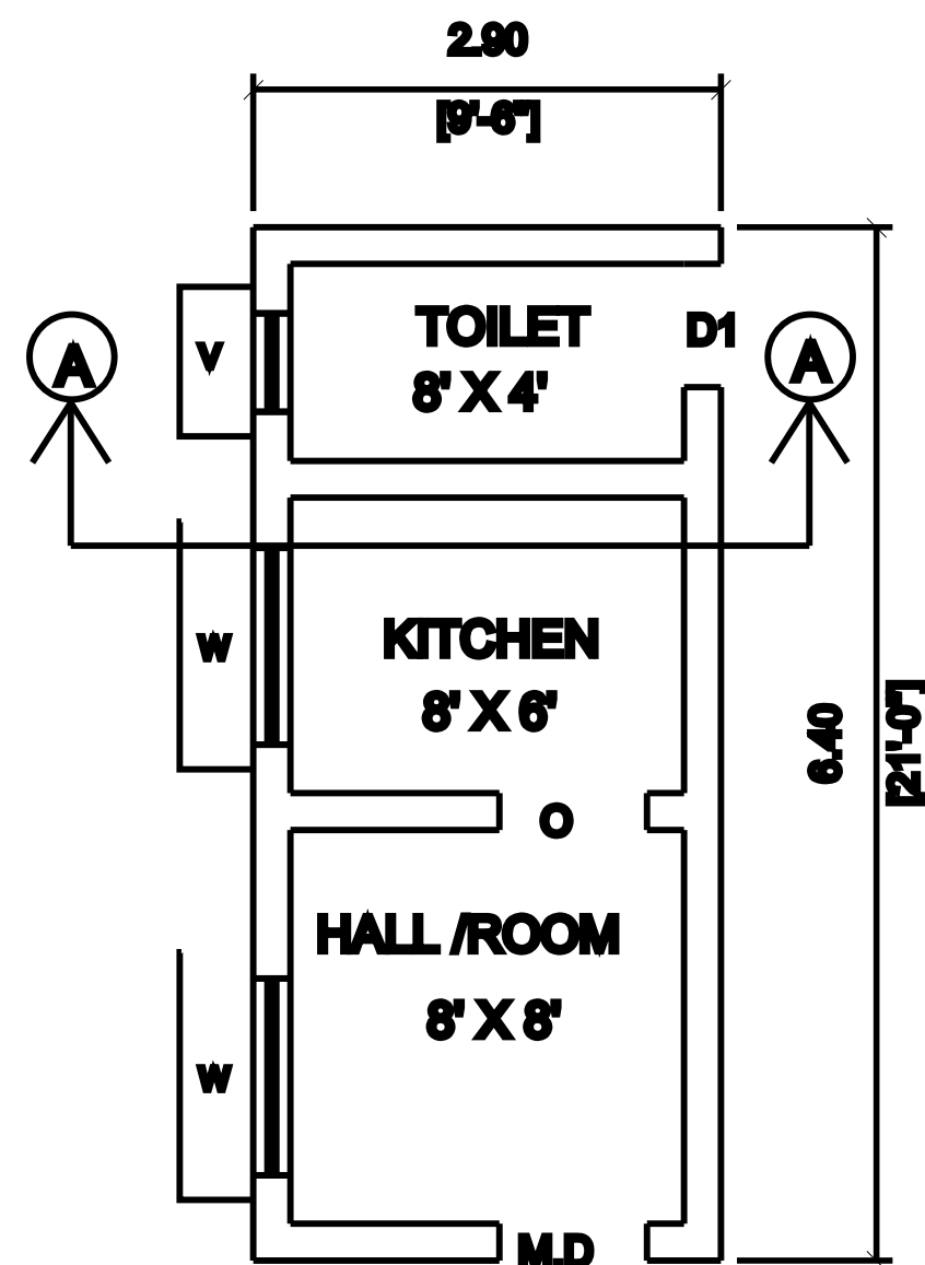
PLAN
