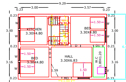
FIRST FLOOR RESIDENTIAL PLAN
