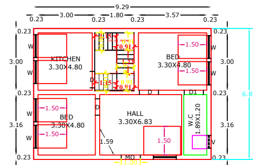
GROUND FLOOR RESIDENTIAL PLAN
