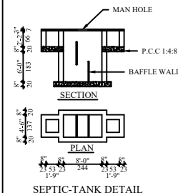
SEPTIC-TANK DETAIL
