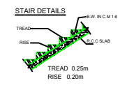
STAIR DETAILS
