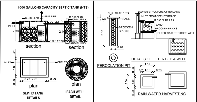
SECTION
