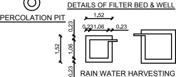
RAIN WATER HARVESTING
