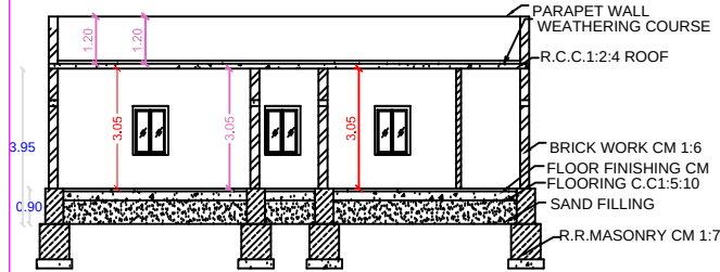
SECTION ON SV
