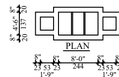
SEPTIC-TANK DETAIL
