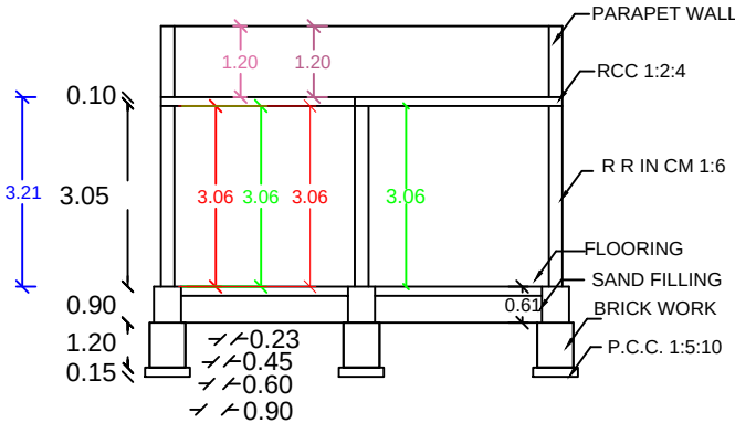
SECTION AB
