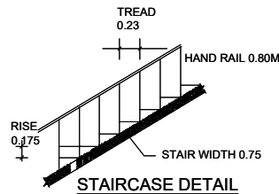
STAIRCASE DETAIL
