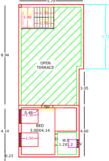
FIRST FLOOR RESIDENTIAL PLAN
