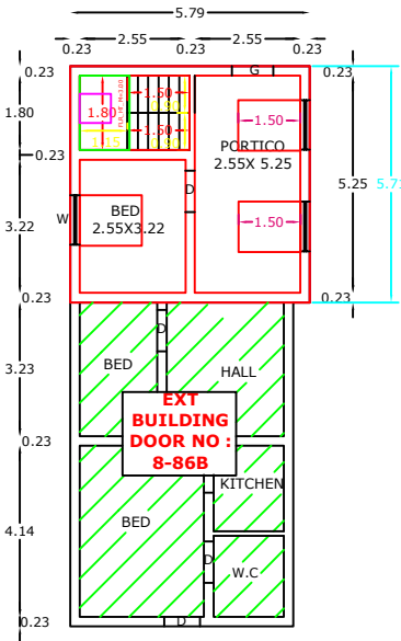
EXT & PRO GROUND FLOOR RESIDENTIAL PLAN
