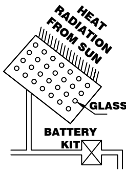
SOLAR SYSTEM
