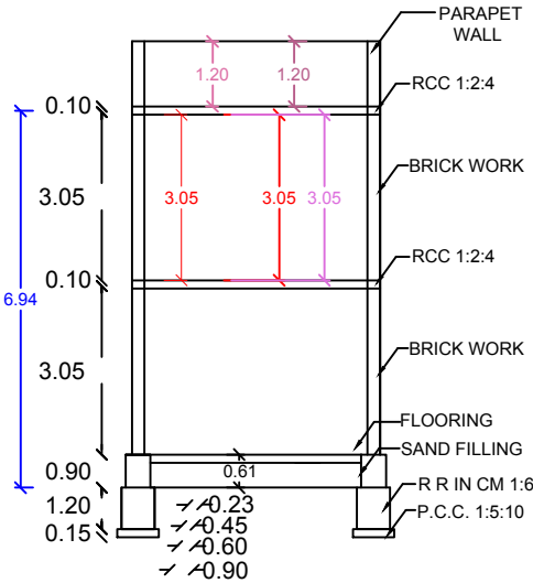
SECTION AB
