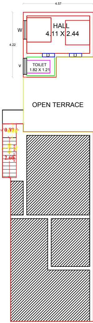
PRO & EXG.FIRST FLOOR PLAN
