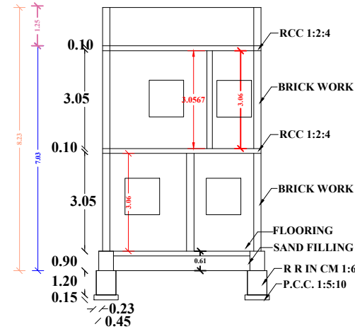
SECTION AB
