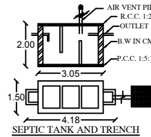
SEPTIC TANK AND TRENCH
