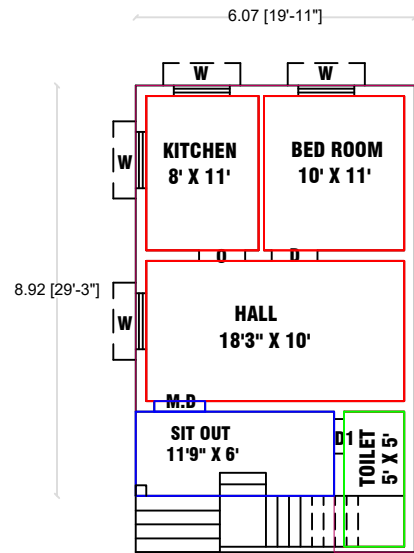
PLAN
