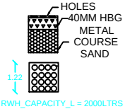
RAIN WATER COLLECTING TANK
