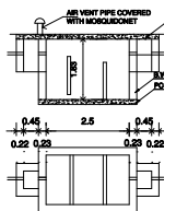
PLAN&SECTION OF SEPTIC TANK
