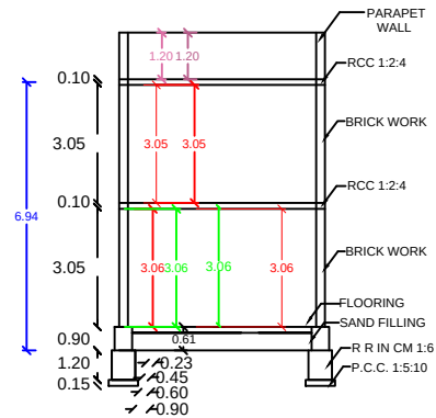
SECTION AB
