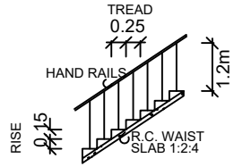
STAIRCASE DETAILS
