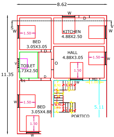
FLOOR
