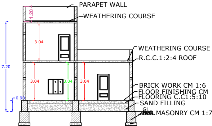
SECTION ON SV
