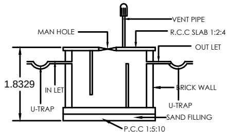
SECTION E.F SEPTIC TANK DETAIL
