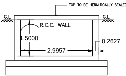
RWH SECTION
