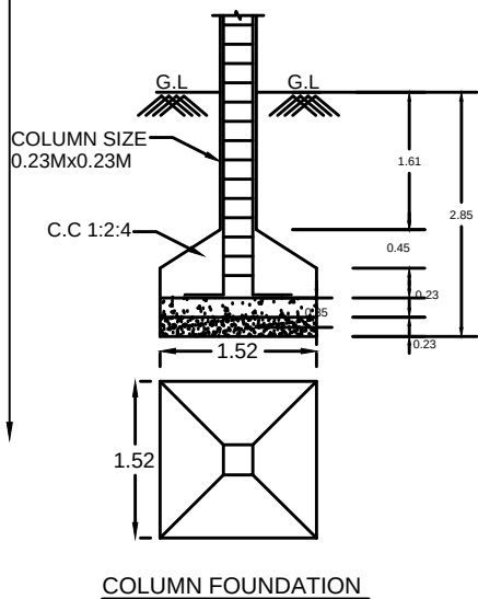
COLUMN FOUNDATION
