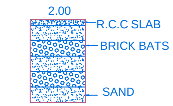
SECTION ON C - D
