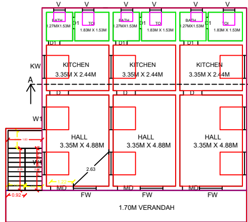
TYPICAL_FLOOR_PLAN=1,2
