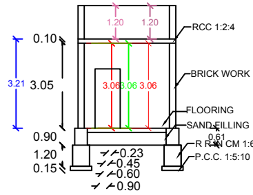
SECTION AB
