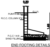
END FOOTING DETAILS
