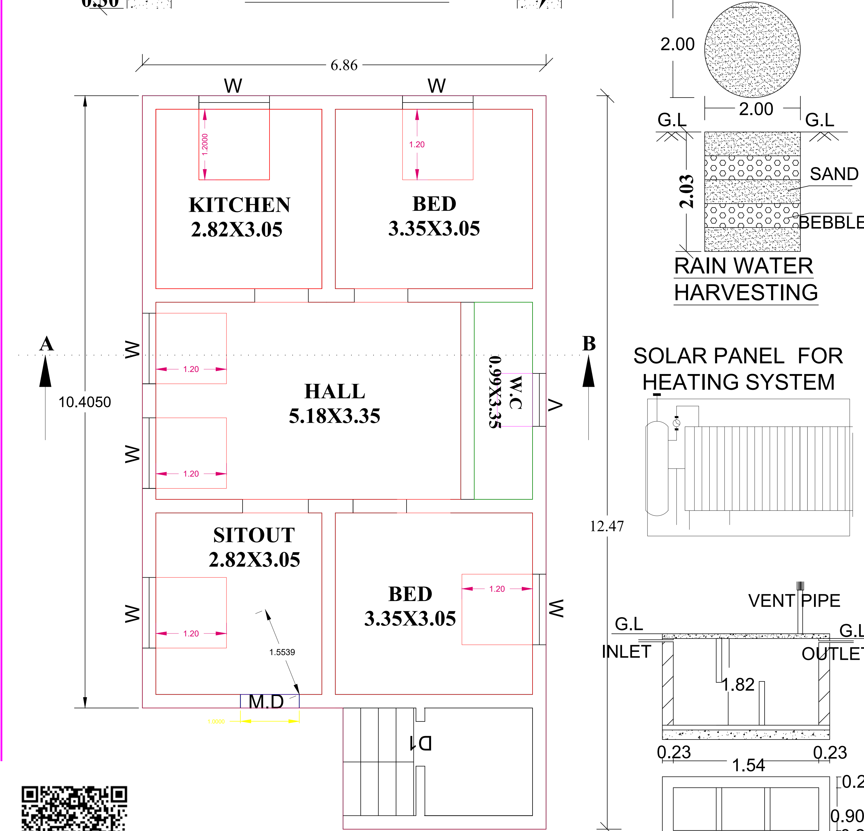
PLAN
