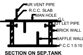
SECTION ON SEPT.TANK
