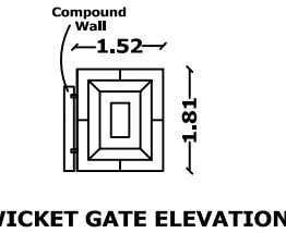
WICKET GATE ELEVATION
