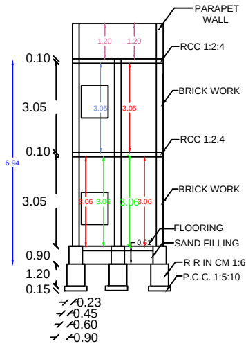
SECTION AB
