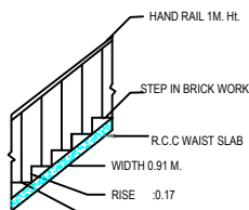
STAIR DETAIL
