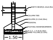
FOUNDATION DETAILS
