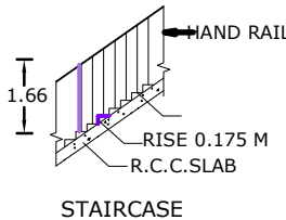
STAIRCASE
