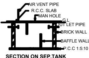
SECTION ON SEPT.TANK
