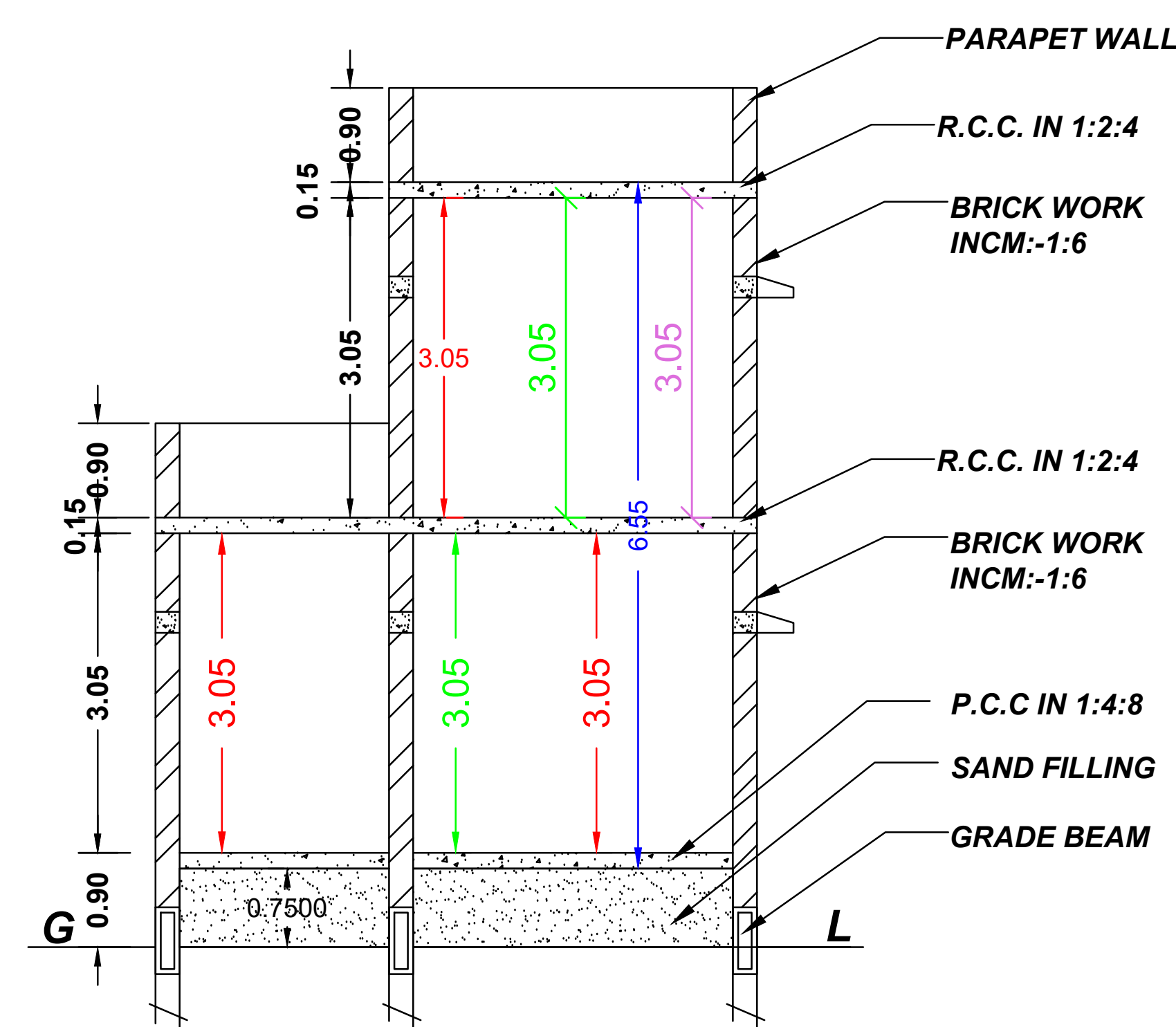
SECTION "AB"
