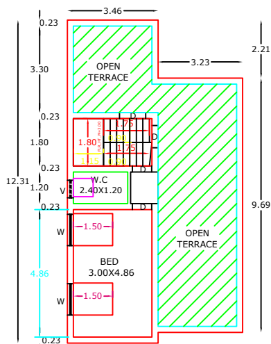
FIRST FLOOR RESIDENTIAL PLAN
