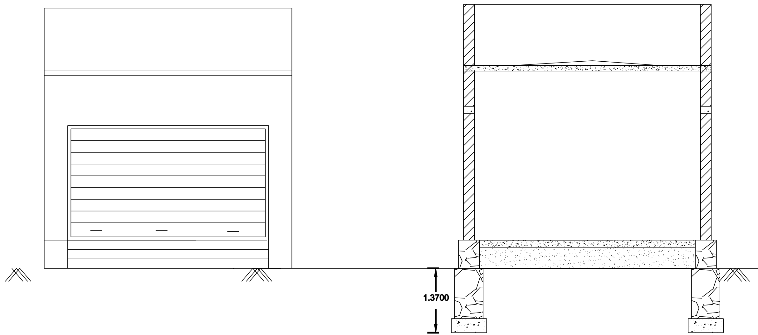
CROSS SECTION
